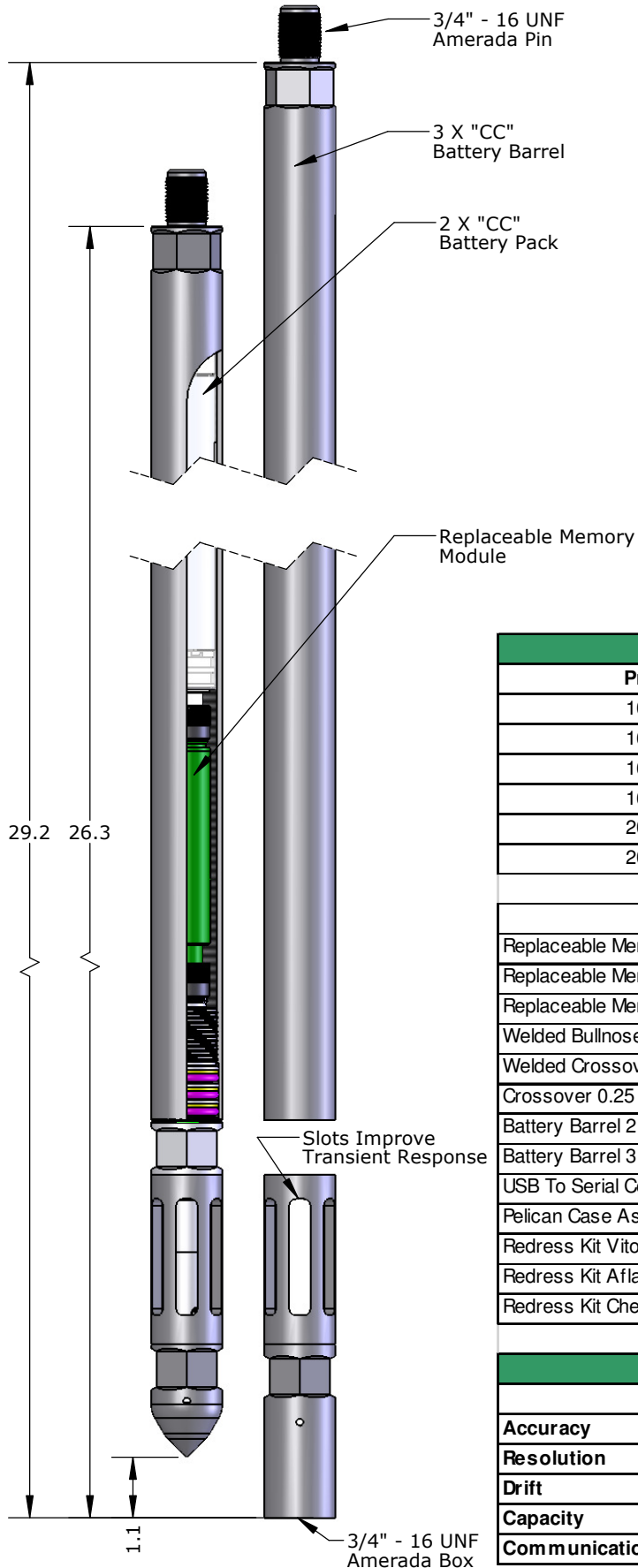
1.25" OD Quartz DXB II Memory Tool - Inconel 718
